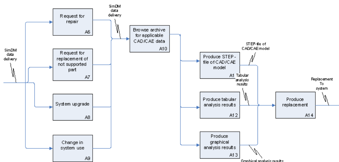
Figure 2: Process diagram - Use in customer support organizations
